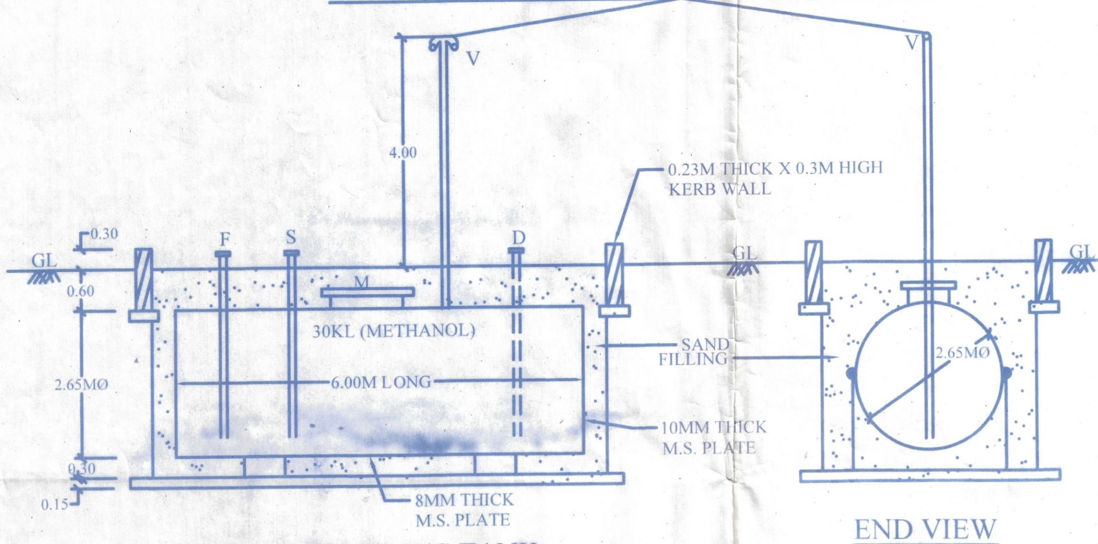
ELEVATION OF U/G TANK
